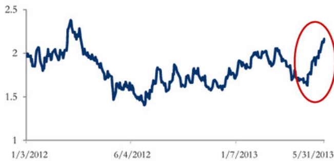
Low Leverage
